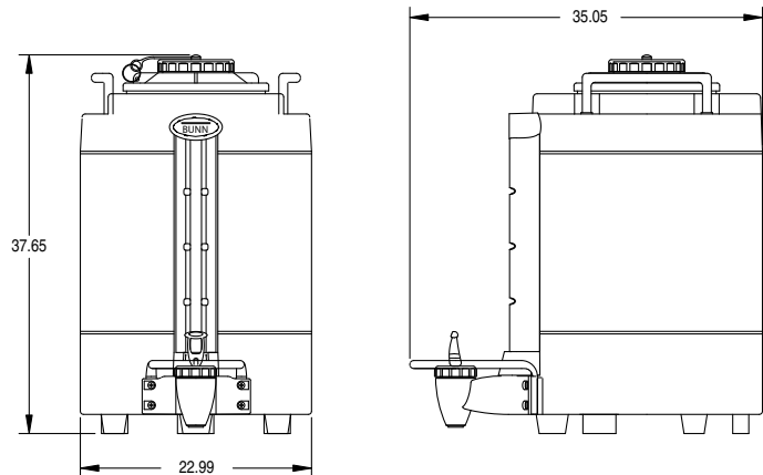
1.5 Gal TF Server
