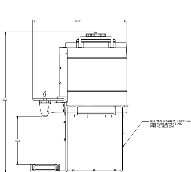
1 Gal TF Server with wire stand
