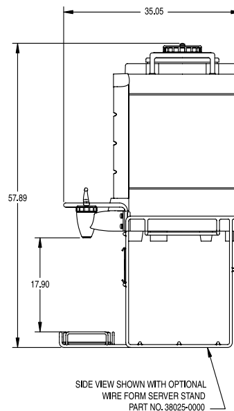
1.5 Gal TF Server with wire stand
