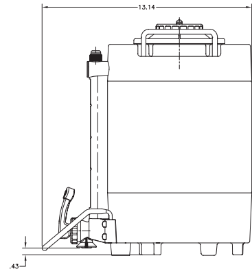
1.5 Gal TF Mechanical Baseless Server
